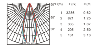
Beam angle 22° Luminous flux: 1063lm
