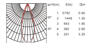
Beam angle 22° Luminous flux: 1688lm
