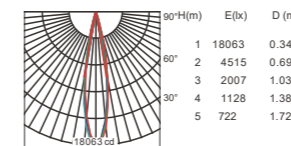
Beam angle 18° Luminous flux: 1710lm
