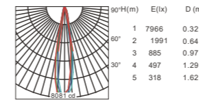
Beam angle 12° Luminous flux: 1163lm
