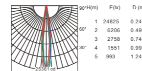
Beam angle 12° Luminous flux: 1562lm
