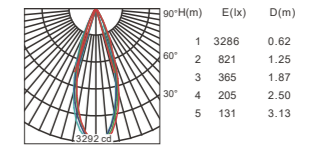
Beam angle 36° Luminous flux: 1204lm
