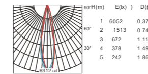
Beam angle 18° Luminous flux: 1200lm
