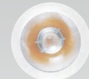
KAS-TL10R-C-80 Power: 25W/30W Diameter: 80mm Cutout: 85-90mm
