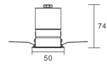
K-CL25-2F-R2D Power: 8W Cutout: 45mm Height: 74mm
