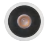
K-CL25-2F-R2D Power: 8W Cutout: 45mm Height: 74mm
