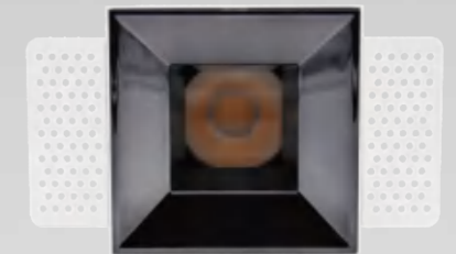
K-CL36-4F-S3D Power: 30W Cutout: 100*100mm Height: 165mm
