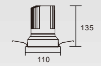
K-CL36-4W-R1S Power: 30W Cutout: 100mm Height: 135mm
