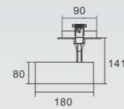
KAS-TL10L-C-80 Power: 25W/30W Diameter: 80mm Cutout: 85-90mm
