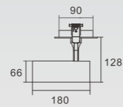
KAS-TL10L-C-66 Power: 10W/15W Diameter: 66mm Cutout: 85-90mm
